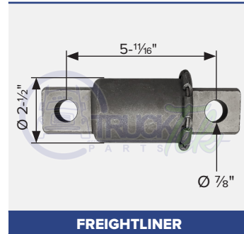
FREIGHTLINER OEM 1616412000 Anti-walk pivot bushing
