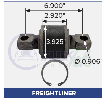
FREIGHTLINER OEM 800480078 Torque V-Rod apex bushing kit (with snap ring)
