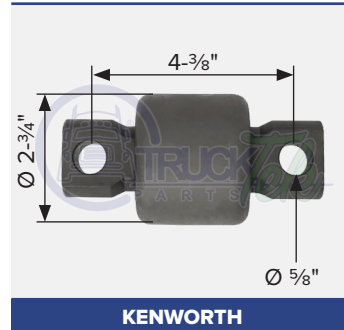
KENWORTH OEM 52375, B656005 2 spring eye hanger bushing
