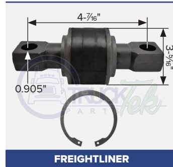
FREIGHTLINER OEM 70480054000 Torque V-Rod apex bushing kit (with snap ring)
