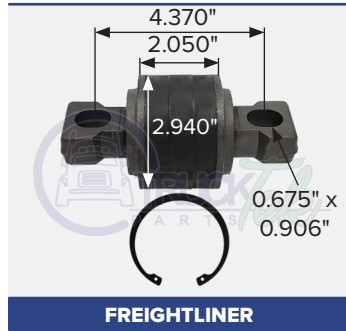
FREIGHTLINER OEM 62480041000, A237903 Torque V-Rod end bushing kit (with snap ring)
