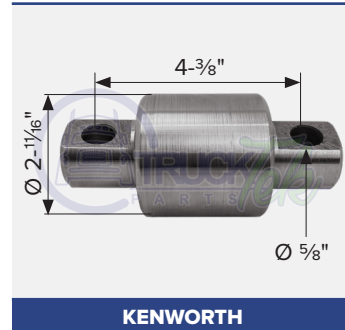
KENWORTH OEM B651006, 52256, 52272 Spring eye hanger bushing 59-502, 59-504, 59-506, 59-518
