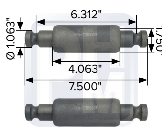
BENDIX OEM 5016364
