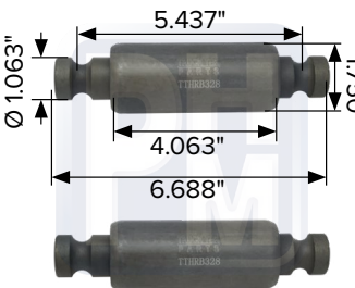
VOLVO OEM 170107796
