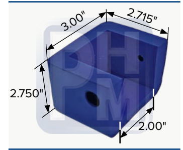
OEM 13-03510, 30.4004R Hood rest center bushing
