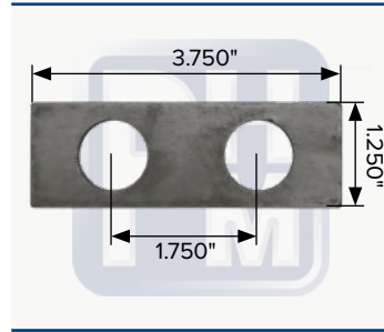
OEM 305114001, MPB341 Alignment shim
