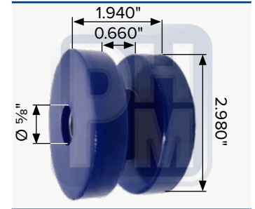
OEM 05-16070-000 Radiator mount (Polyurethane) Century, Columbia
