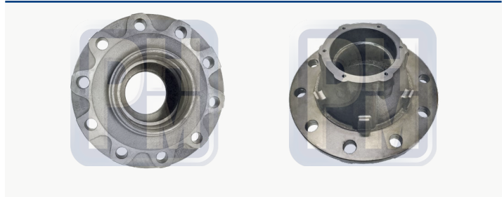
Maza remolque 10 barrenos Outboard mount drum-serrated unimount Bolt 11 1/4"
