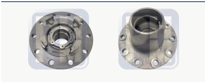
Maza delantera Para birlo unimount Front hub Bolt 11 1/4"
